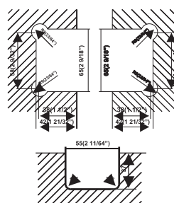
Hole Dimension Of Glass
