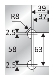
Hole Dimension Of Glass
