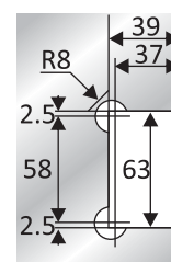
Hole Dimension Of Glass
