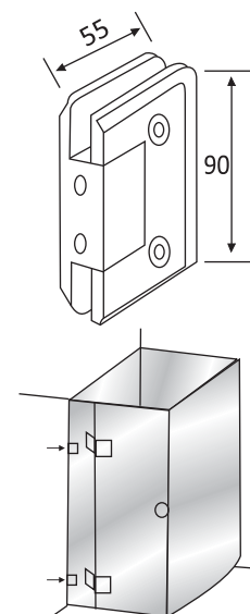
Hole Dimension Of Glass
