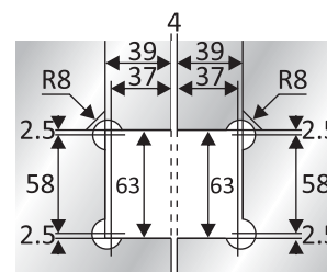
Hole Dimension Of Glass
