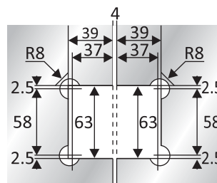
Hole Dimension Of Glass
