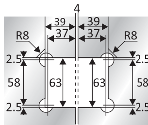
Hole Dimension Of Glass
