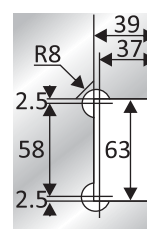
Hole Dimension Of Glass
