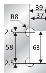
Hole Dimension Of Glass
