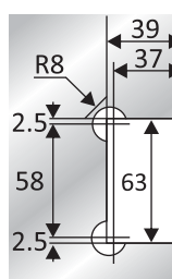
Hole Dimension Of Glass
